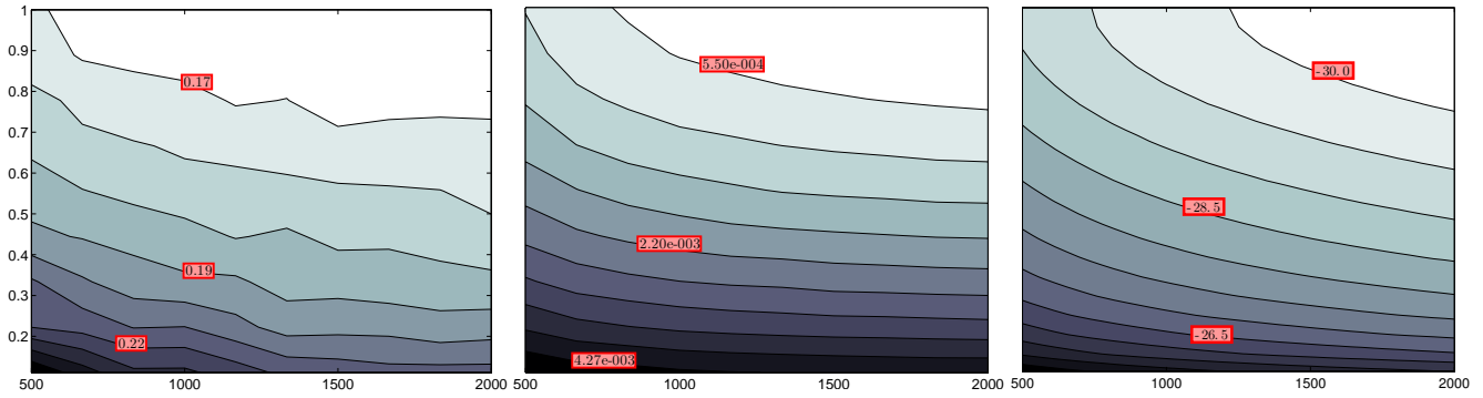
Figure 1. Three error measures for the multinomial naive Bayes SSL classifier applied to Reuters RCV1 text data. In each, error is a function of n (horizontal axis) and \lambda (vertical axis). The left depicts classification error rate, the middle depicts the trace of empirical mse, and right depicts the log-trace of the asymptotic variance. Results were obtained using held-out sets and averaged using cross validation. Particularly noteworthy is a striking correlation among all three figures, justifying the use of asymptotic variance as a surrogate for classification error, even for relatively small values of n .
